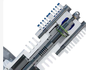
Fourth stage in tempered steel with 6 piston rings in special cast iron
