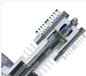
Fourth stage in tempered steel with 6 piston rings in special cast iron
